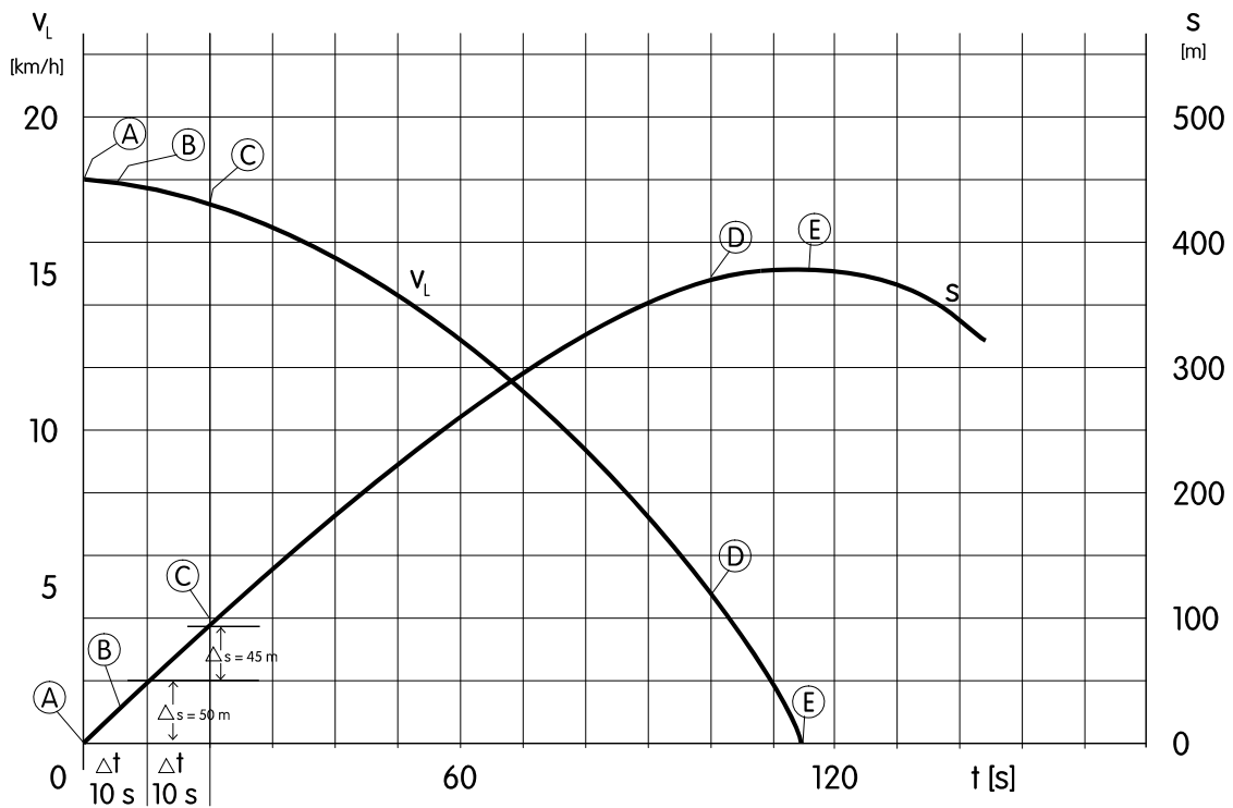
Figure 1: Stopping manoeuvre
