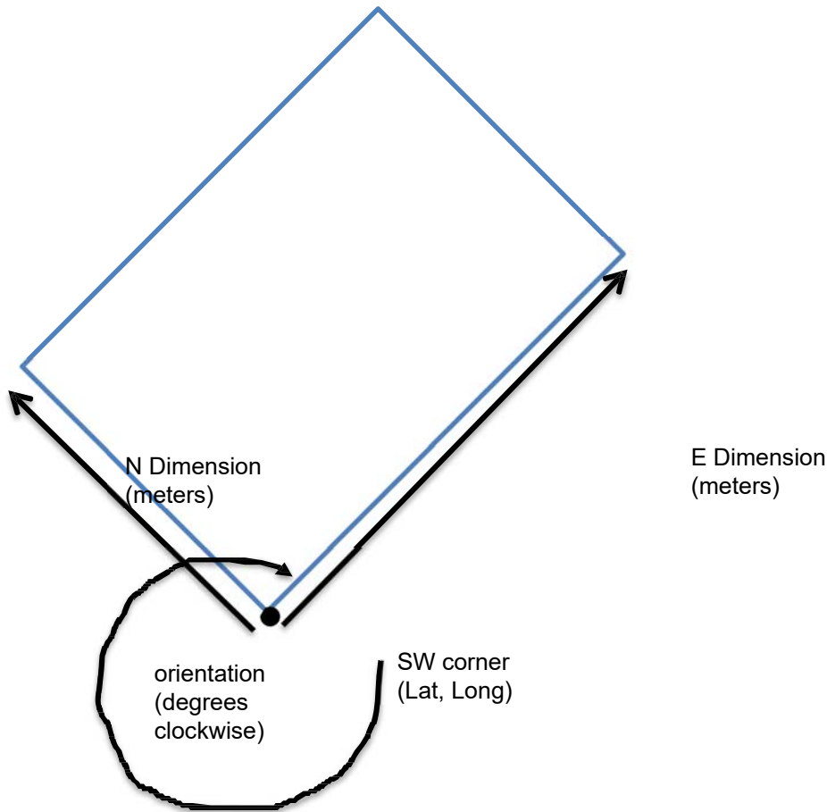
Figure 15-5 Rectangle Diagram
