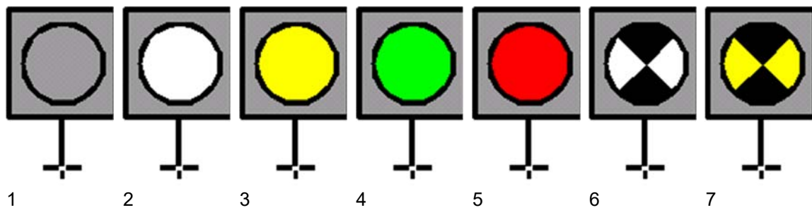
Figure 15-2 Light Status
